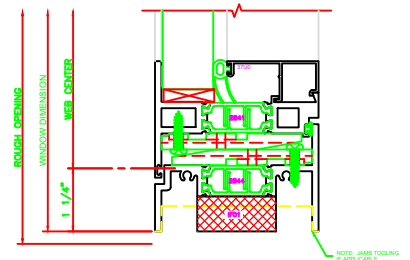
241 SILL 325 CASEMENT OUT BUTT HINGES
